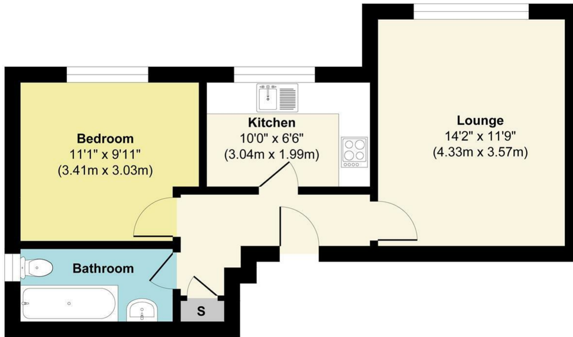
Floor Plan
