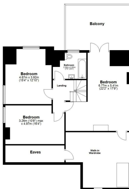
Second Floor Approx. 107.6 sq. metres (1158.7 sq. feet)
