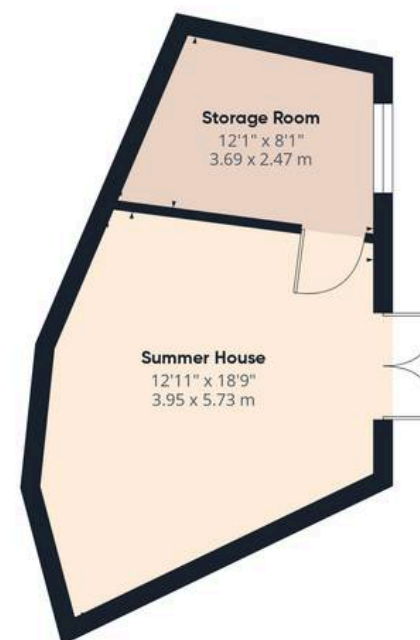
Ground Floor Building 2
