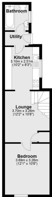
Ground Floor Approx. 37.7 sq. metres (408.1 sq. feet)
