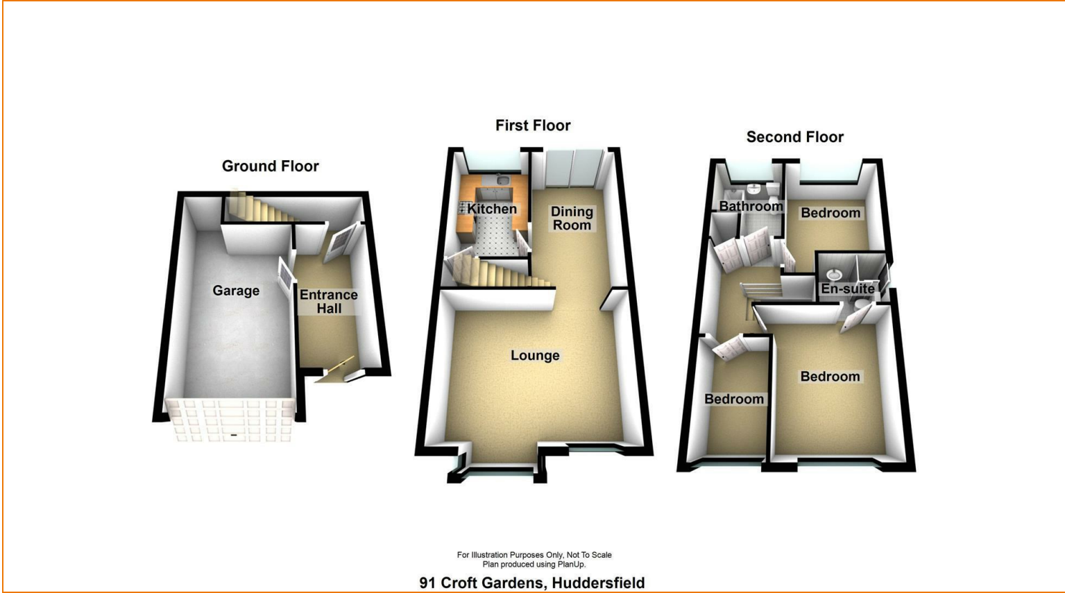
Floor Plan
