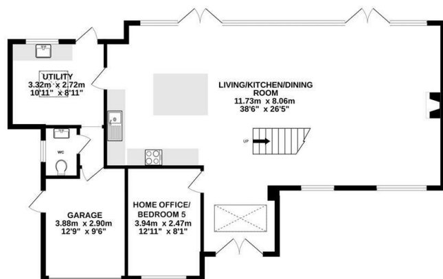
GROUND FLOOR 104.5 sq.m. (1125 sq.ft.) approx.
