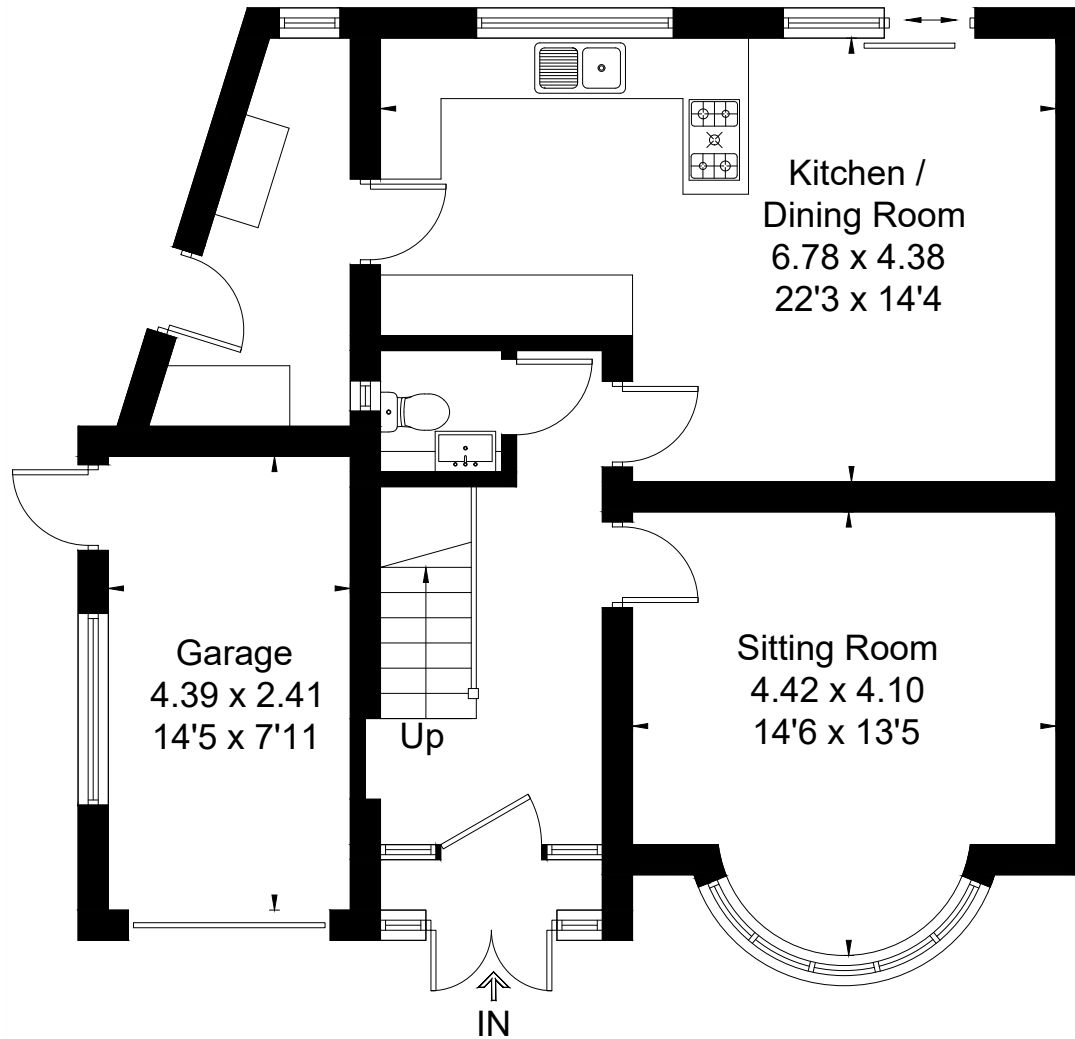
Ground Floor
