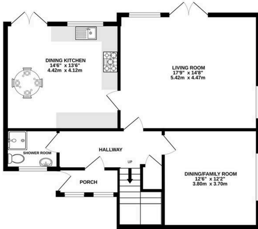
GROUND FLOOR 777 sq.ft. (72.2 sq.m.) approx.
