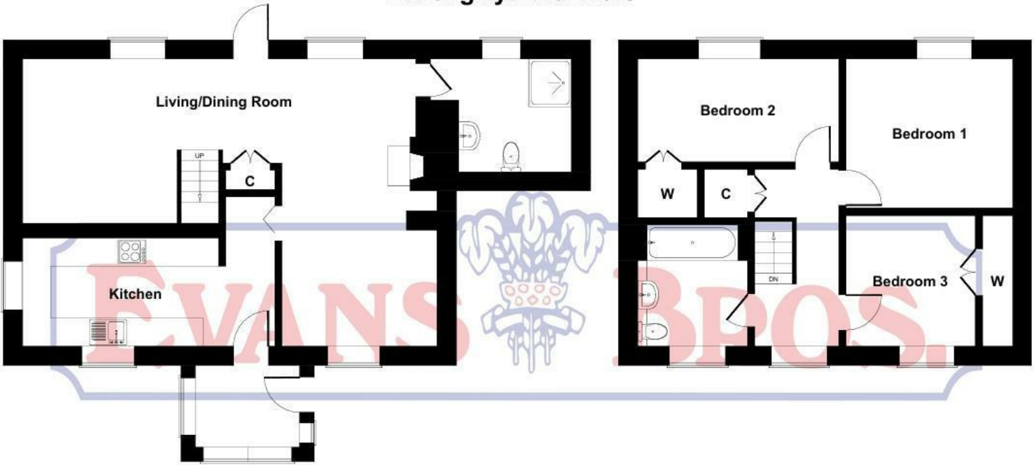
GROUND FLOOR
