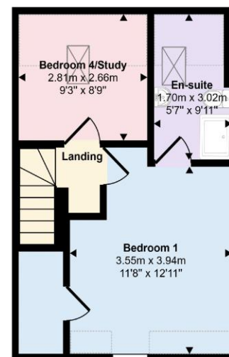
Second Floor Approx 33 sq m / 358 sq ft
