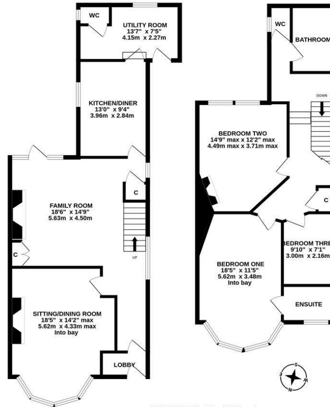
TOTAL FLOOR AREA: 1440 sq.ft. (133.8 sq.m.) approx.
