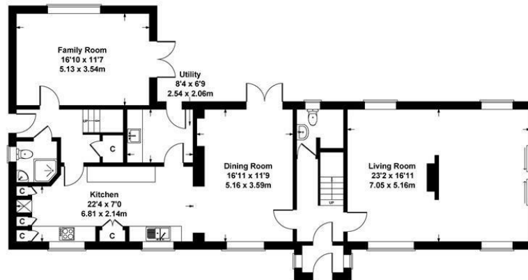
GROUND FLOOR
