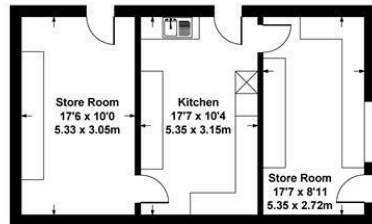
OUTBUILDING
