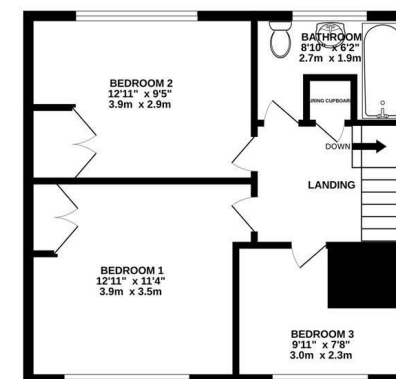
1ST FLOOR 438 sq.ft. (40.7 sq.m.) approx.
