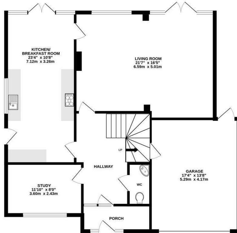
GROUND FLOOR 1124 sq.ft. (104.4 sq.m.) approx.
