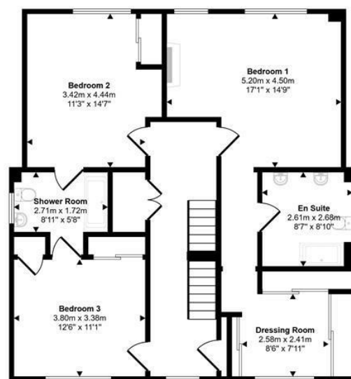
First Floor Approx 101 sq m / 1088 sq ft
