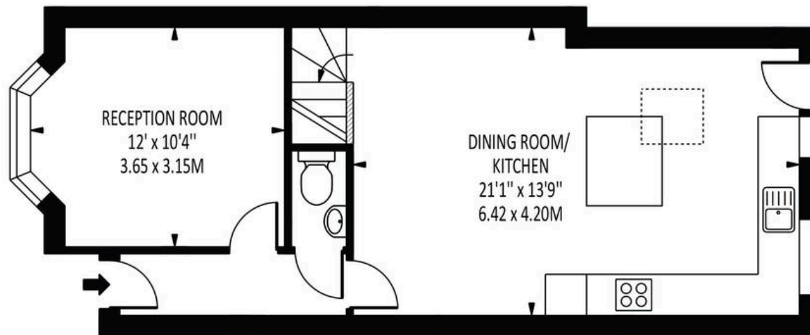
GROUND FLOOR
