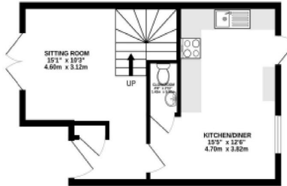
GROUND FLOOR 356 sq.ft. (33.0 sq.m.) approx.
