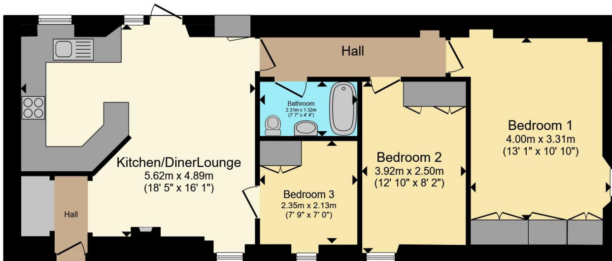
Floor Plan
