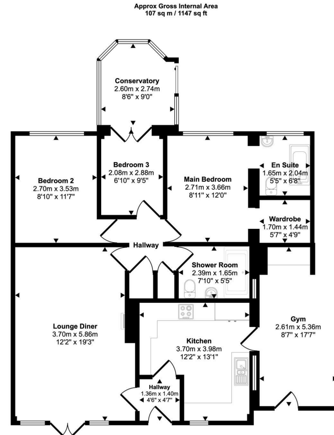
Floorplan
