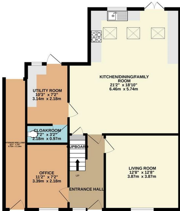
GROUND FLOOR 864 sq.ft. (80.3 sq.m.) approx.
