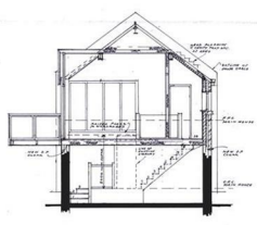
CROSS SECTION A-A
