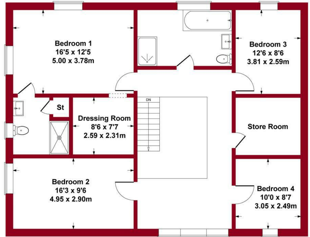
FIRST FLOOR (PLOT 1)
