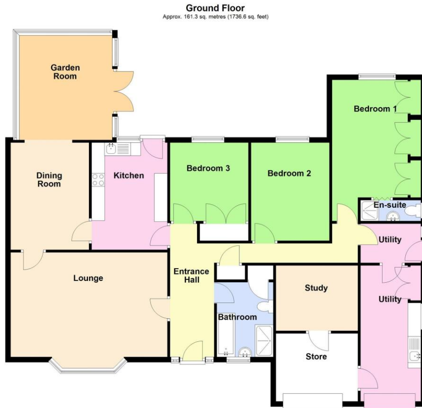
Total area: approx 161.3 sq. metres (1736.6 sq. feet)
