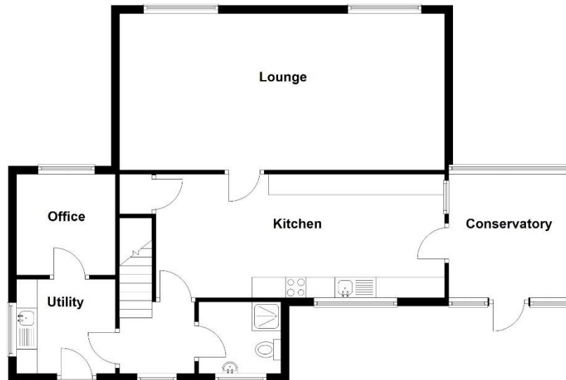
Ground Floor Approx. 82.0 sq. metres (882.4 sq. feet)
