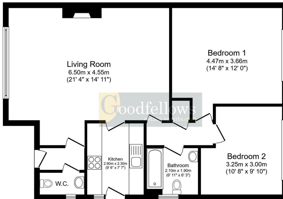
Floor Plan Floor area 80.2 sq.m. (864 sq.ft.)
