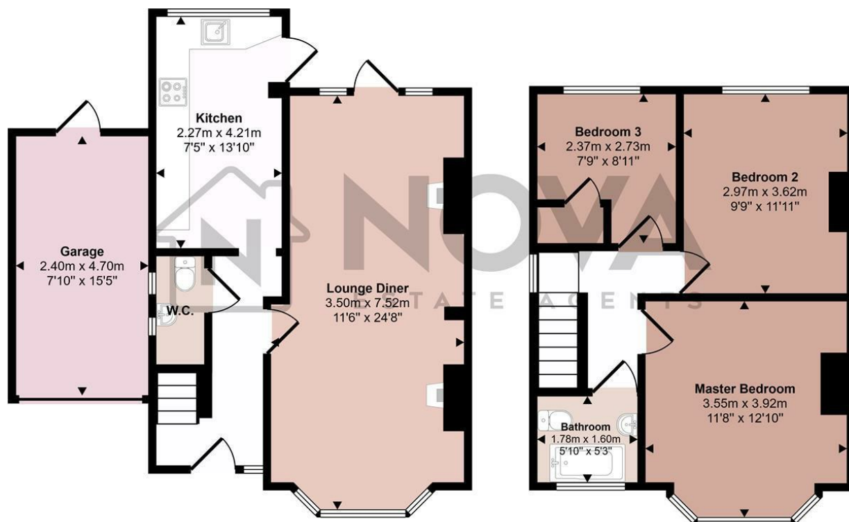
Ground Floor Approx 55 sq m / 592 sq ft
