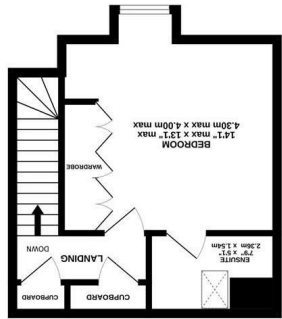
2ND FLOOR 284 sq.ft. (26.4 sq.m.) approx.
