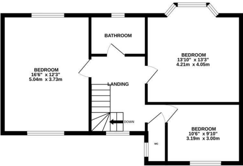
1ST FLOOR 617 sq.ft. (57.3 sq.m.) approx.
