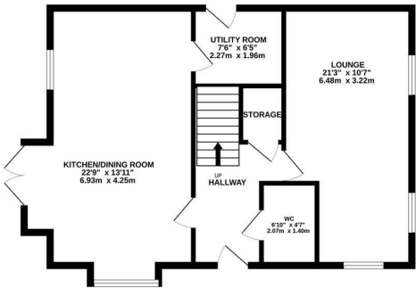
GROUND FLOOR 659 sq.ft. (61.2 sq.m.) approx.
