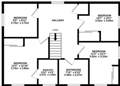
1ST FLOOR 635 sq.ft. (59.0 sq.m.) approx.
