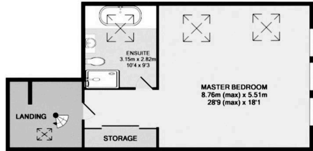
1ST FLOOR APPROX. FLOOR AREA 54.6 SQ. M. (588 SQ. FT.)
