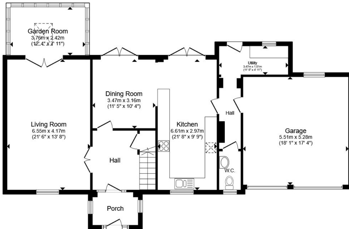
Ground Floor
