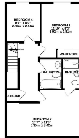
2ND FLOOR
