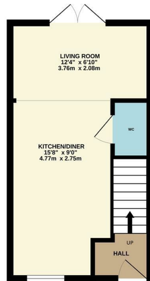
GROUND FLOOR 277 sq.ft. (25.7 sq.m.) approx.
