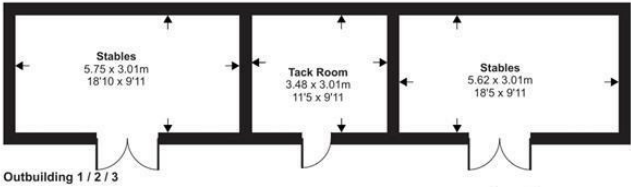
Outbuilding 1 / 2 / 3
