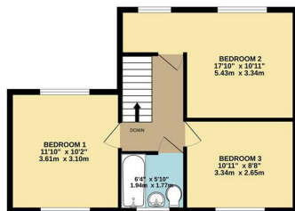
1ST FLOOR 482 sq.ft. (44.8 sq.m.) approx.
