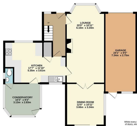
TOTAL FLOOR AREA: 1404 sq.ft. (130.4 sq.m.) approx.
