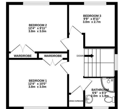
1ST FLOOR 468 sq.ft. (43.5 sq.m.) approx.
