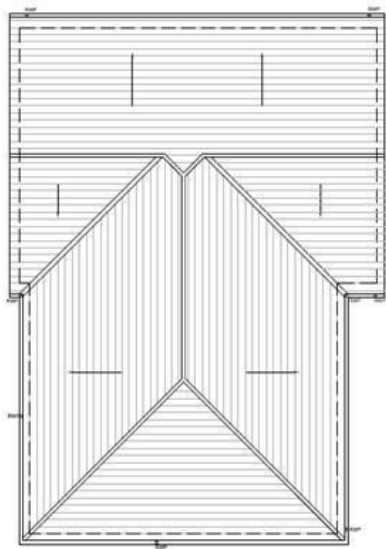
Roof Plan Scale A3 @ 1:100
