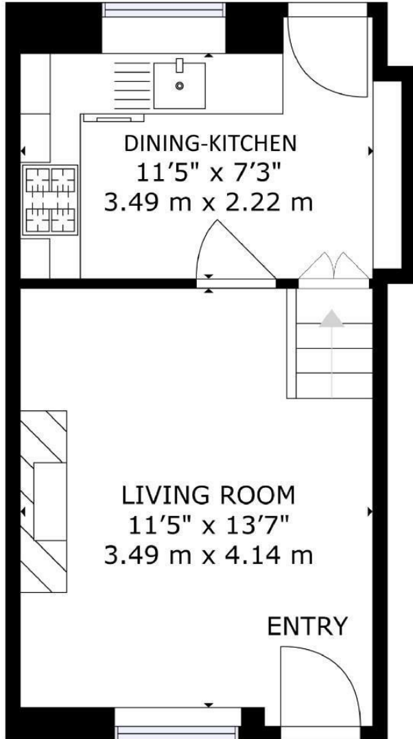
FLOOR 1
