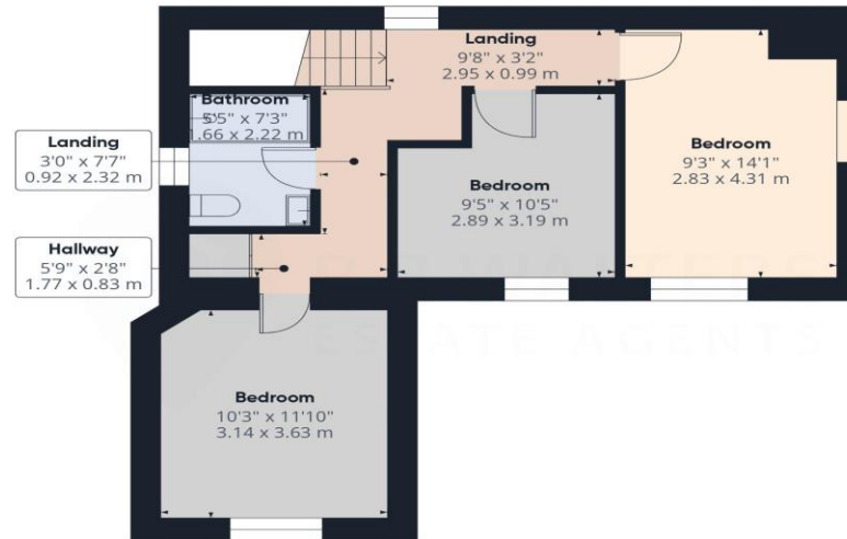
Floor 1 Building 1
