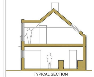
TYPICAL SECTION
