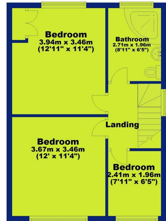
First Floor Approx. 42.6 sq. metres (458.4 sq. feet)
