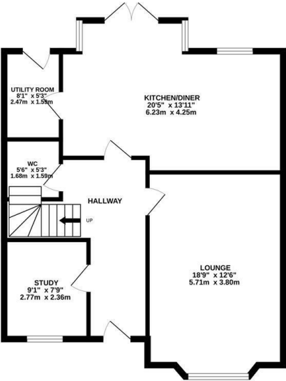
GROUND FLOOR 742 sq.ft. (68.9 sq.m.) approx.
