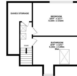
2ND FLOOR 538 sq.ft. (50.0 sq.m.) approx.
