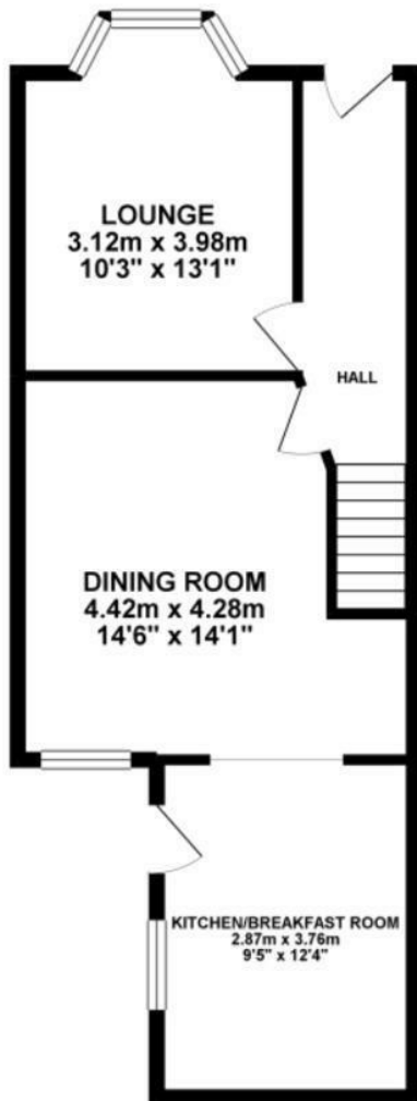
GROUND FLOOR 45.54 sq. m. ( 490.15 sq. ft. )
