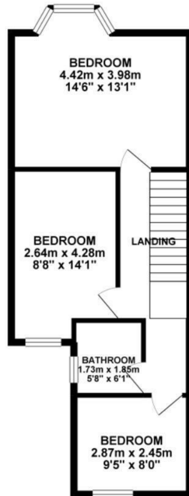
1ST FLOOR 45.54 sq. m. ( 490.22 sq. ft. )
