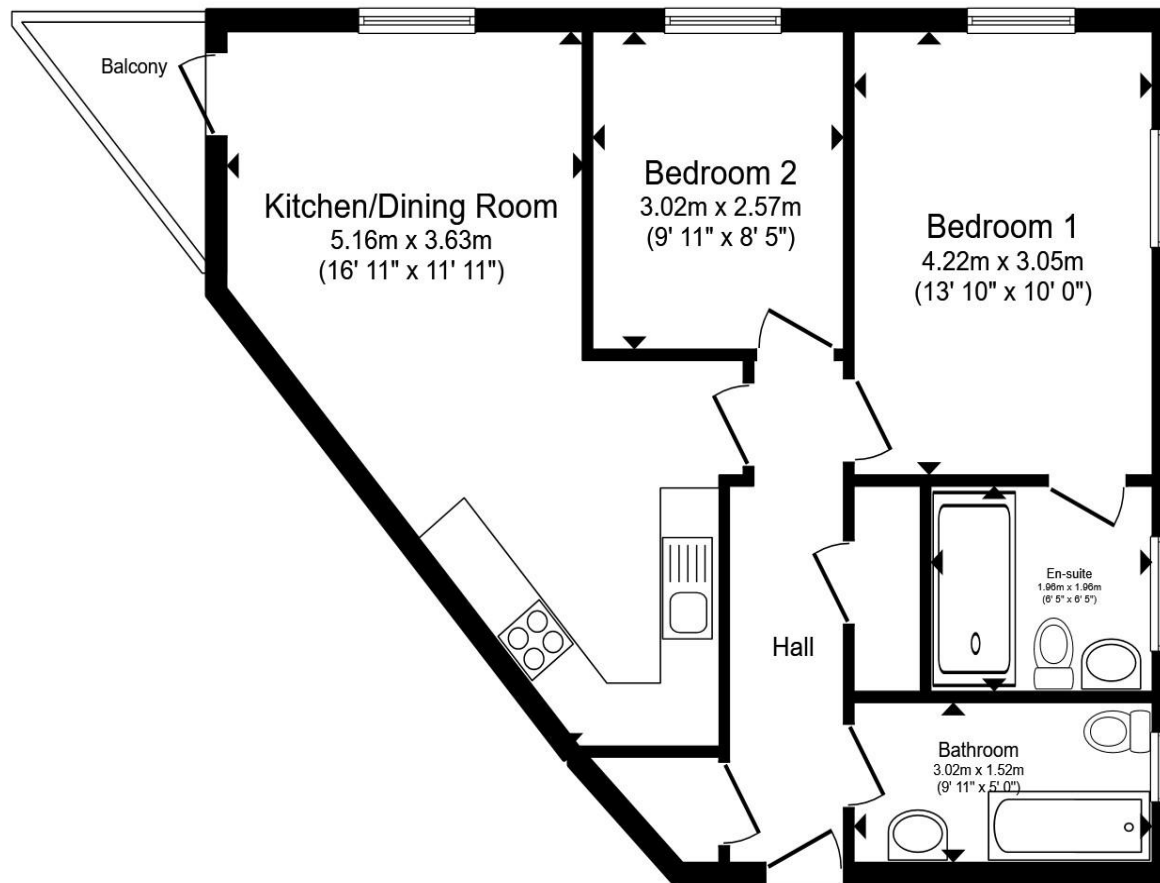
Floor Plan
