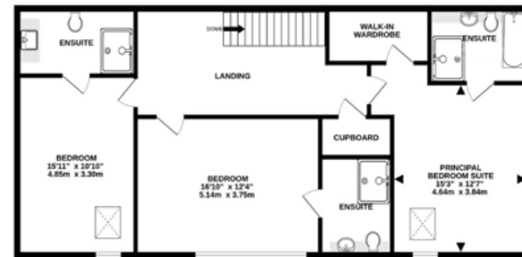
1ST FLOOR 1094 sq.ft. (101.1 sq.m.) approx.
