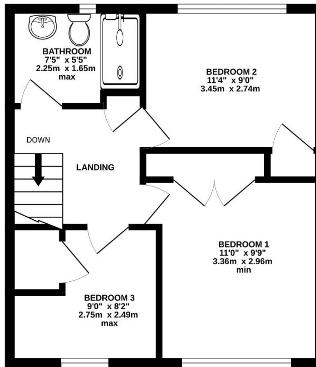
1ST FLOOR 399 sq.ft. (37.1 sq.m.) approx.
