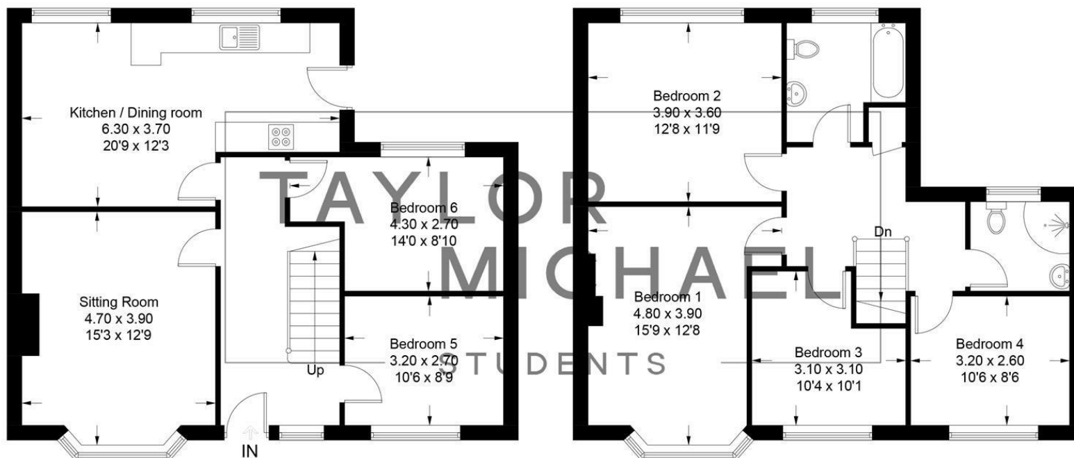
Ground Floor
