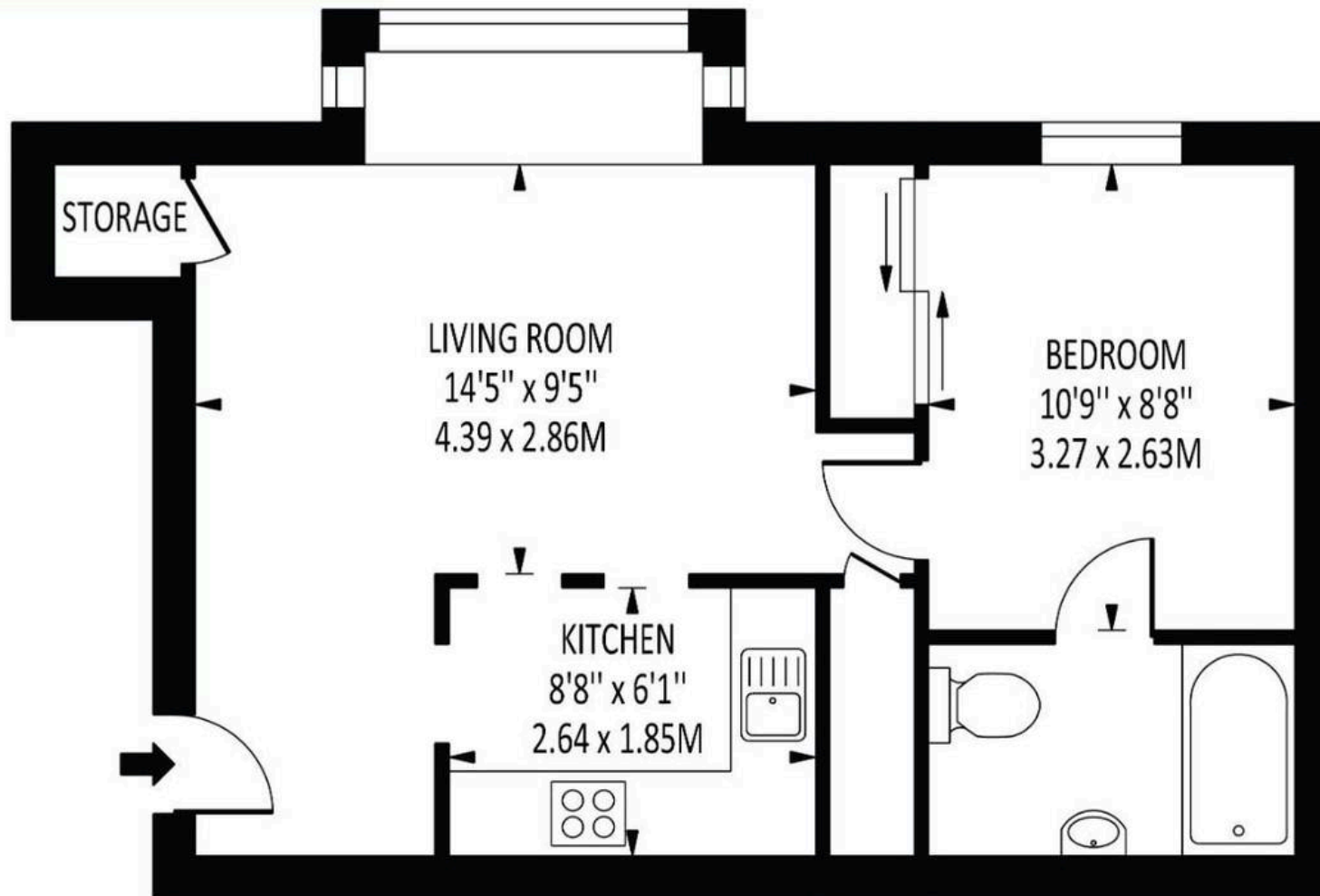
FIRST FLOOR
