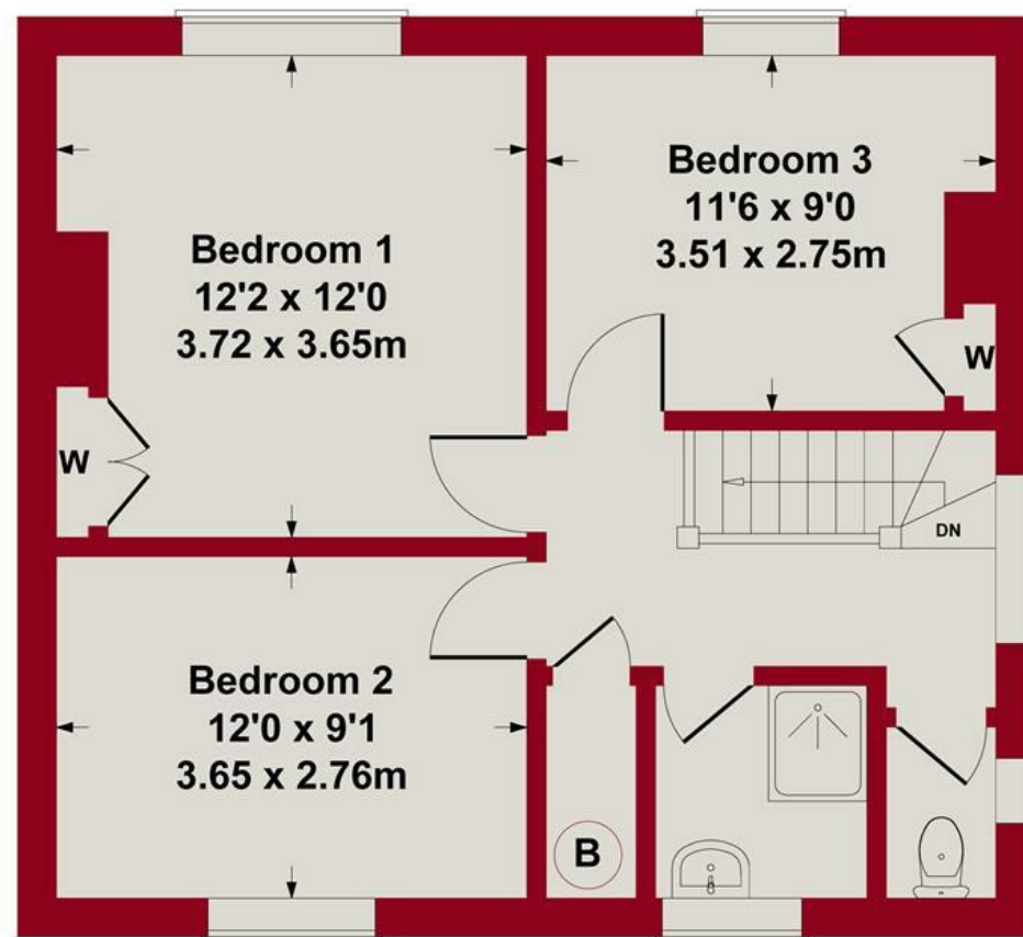
FIRST FLOOR
